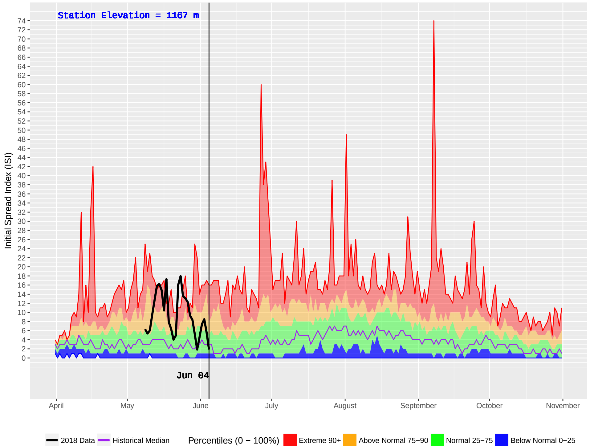
LEIGHTON LAKE (307) : Historical (1982–2016) and Current (2018) Noon Initial Spread Index (ISI)
