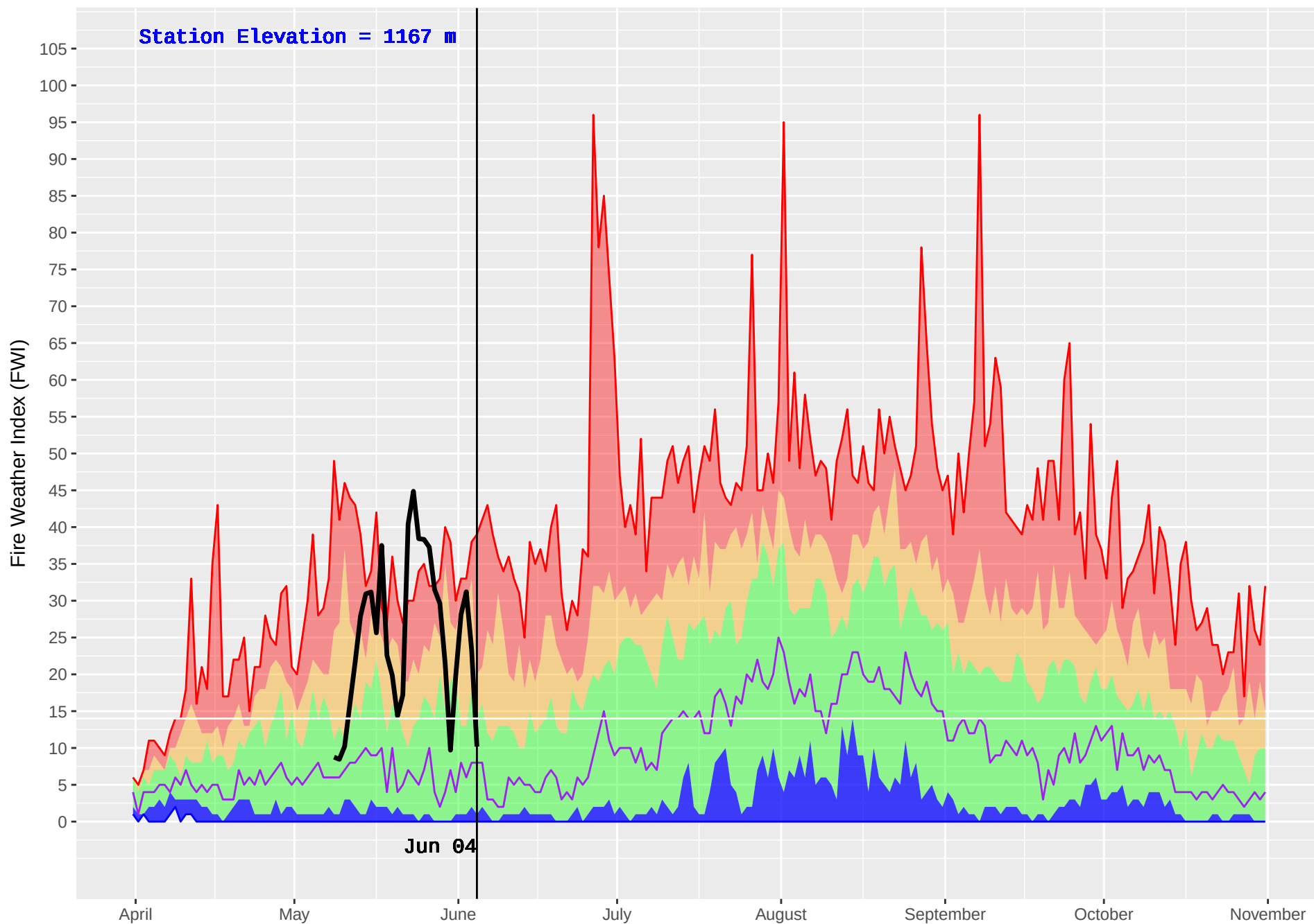
LEIGHTON LAKE (307) : Historical (1982–2016) and Current (2018) Noon Fire Weather Index (FWI)
