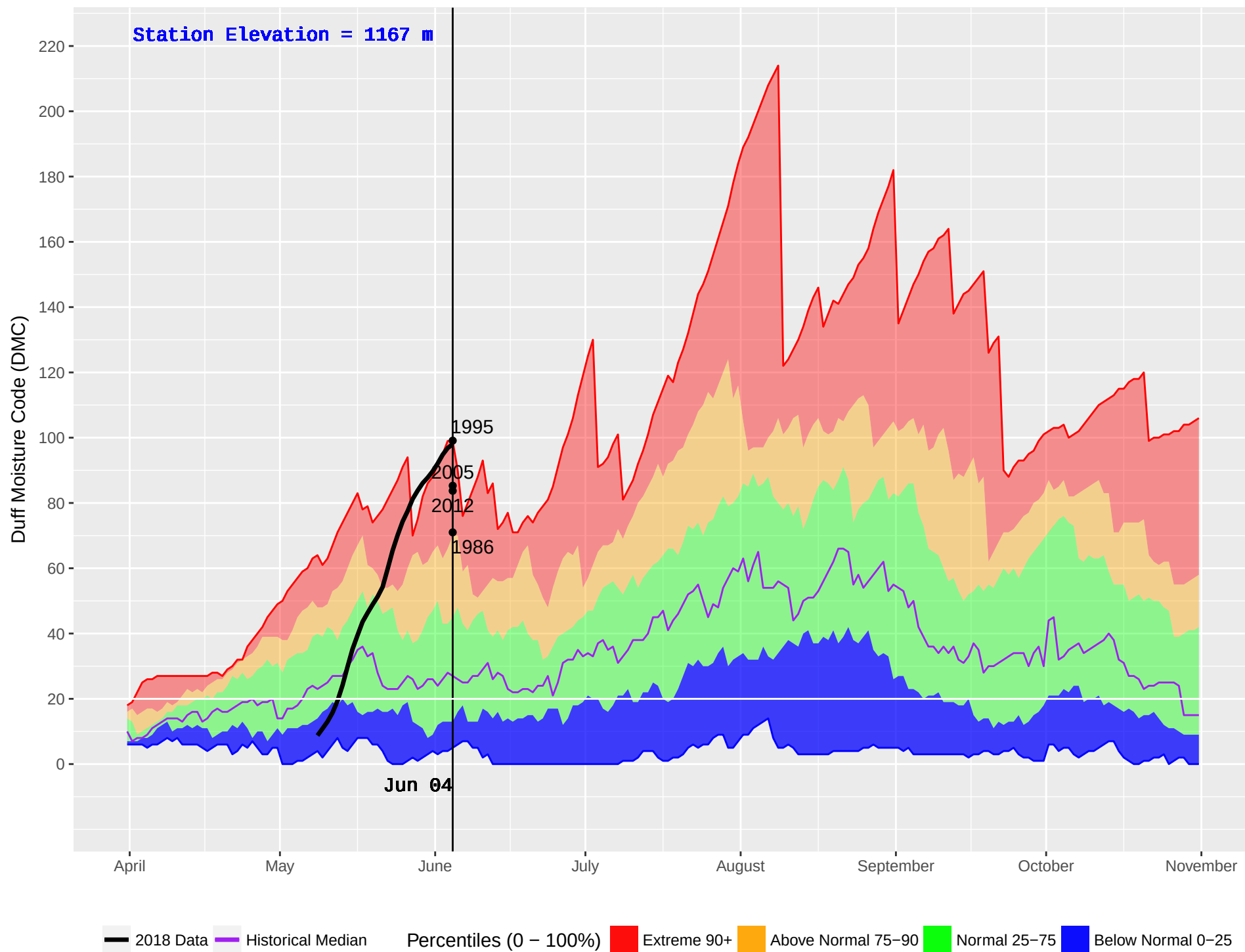
LEIGHTON LAKE (307) : Historical (1982–2016) and Current (2018) Noon Duff Moisture Code (DMC)
